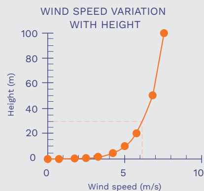
FIGURE 4 Example of wind speed gradient.
