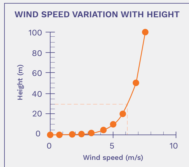
FIGURE 4 Example of wind speed gradient
